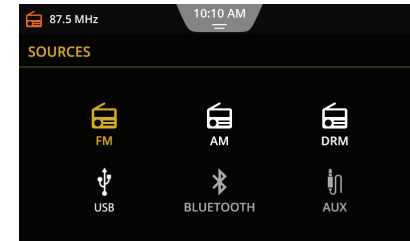
Figure 35: Sources Screen
