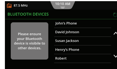
Figure 38: Available Devices
