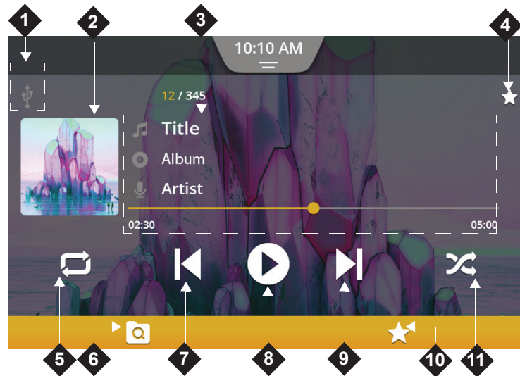
Figure 55: Media Screen
