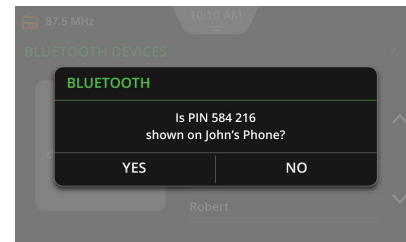
Figure 40: PIN Verification
